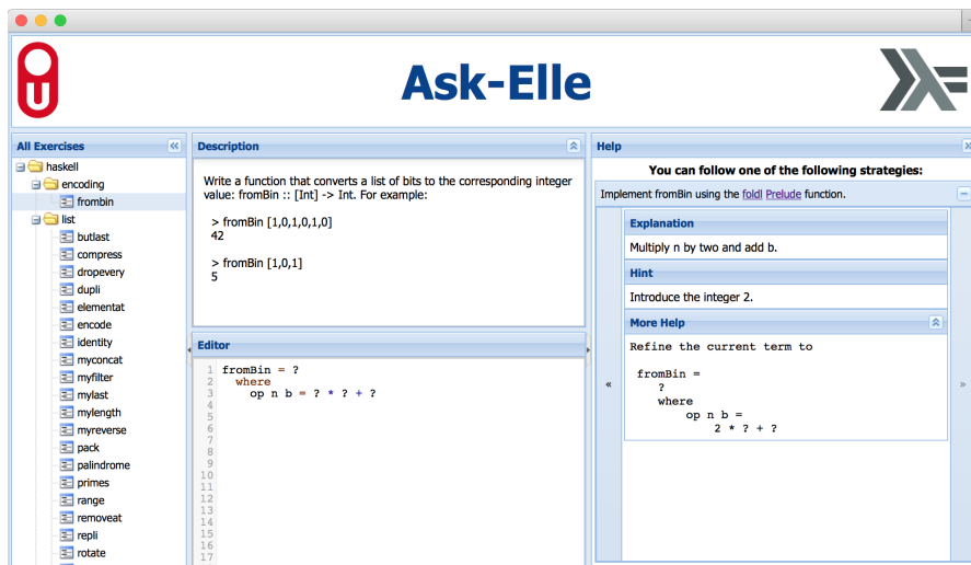
Figure 1 The web-based functional programming tutor
