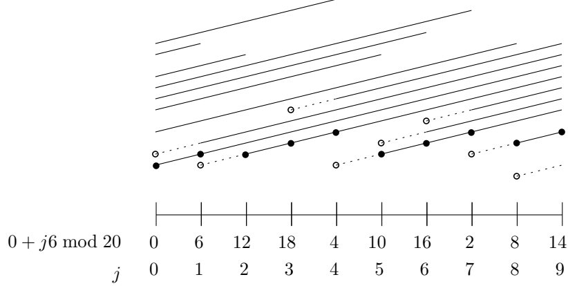
Figure 3: A possible lower envelope used for the set q_0 , with k = 20 and \ell_i = 6 . The empty circles show values in D_{i-1} and the filled disks show values in D_i .
