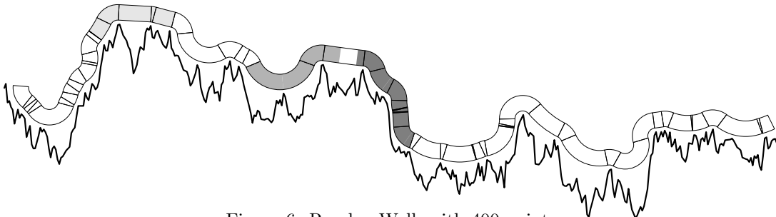
Figure 6: RandomWalk with 400 points
