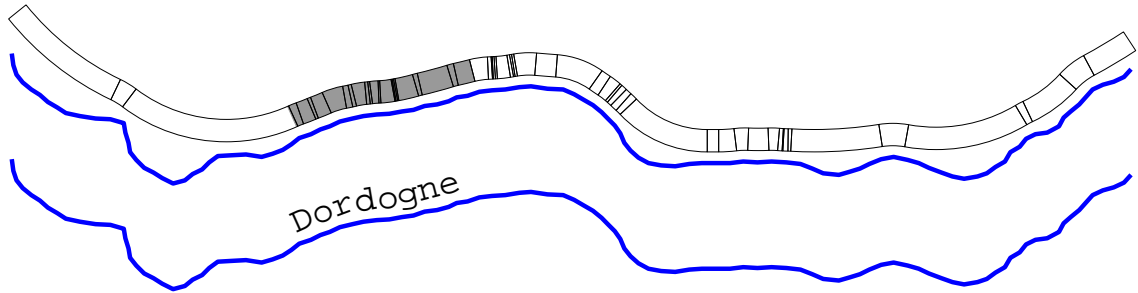
Figure 4: A piece of the Dordogne (109 points). Above with candidate strip and label placement (shaded grey), below with lettering
