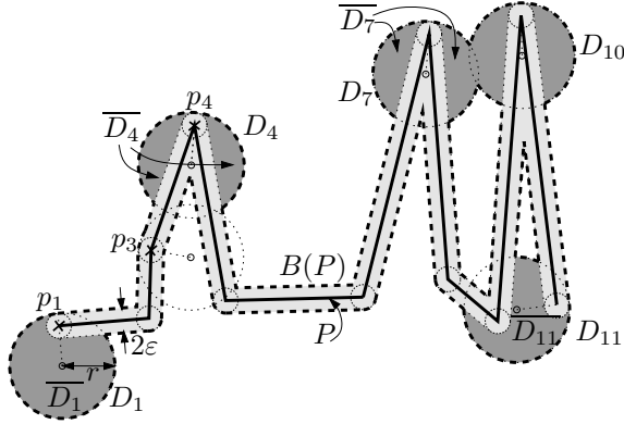
Figure 1: The boundary of the (\varepsilon, r) -buffer B(P) (bold dashed line) of the input polyline P (bold solid line).
