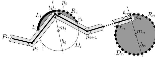
Figure 2: Placing r -disks D_i at right turns p_i of the input polyline P .
