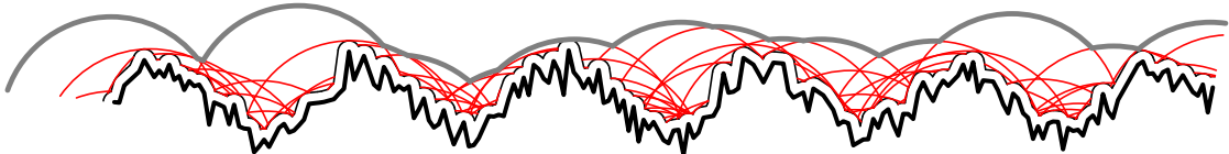
Figure 9: Disturbing effects of the definition of the (\varepsilon, r) -buffer. (The upper part of its outer face is marked by bold grey arcs; the input polyline below consists of bold black line segments.)
