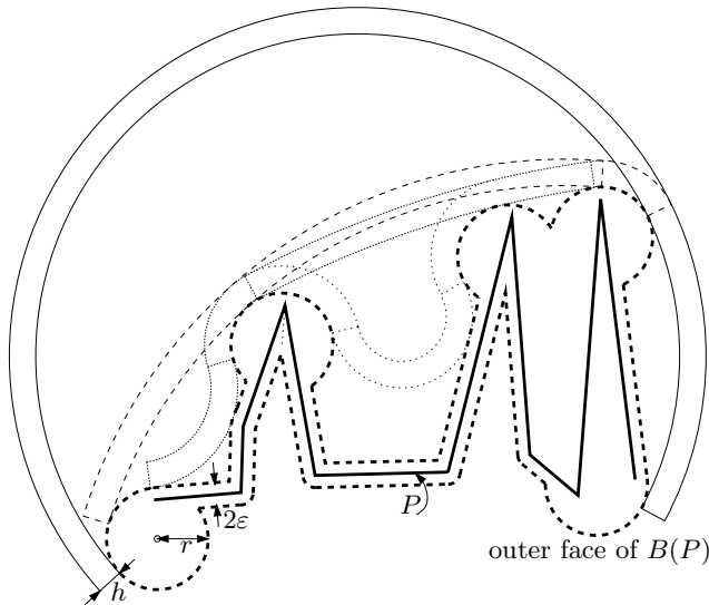
Figure 3: refining the candidate strip: first level (solid), second level (dashed), third level (densely dotted), and fourth level (dotted)
