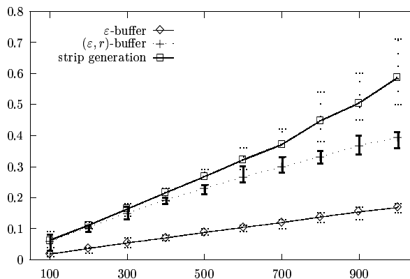
Figure 7: Strip generation time
