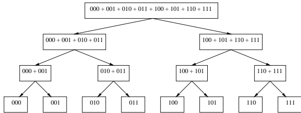
Figure 1: Binary tree partitioning of the Walsh coefficients.
