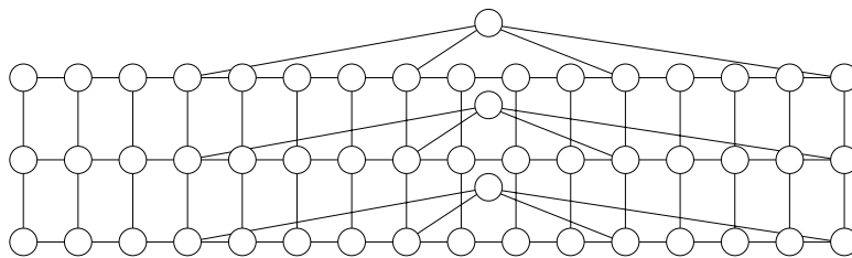
Figure 1: Grid with added vertices z_i
