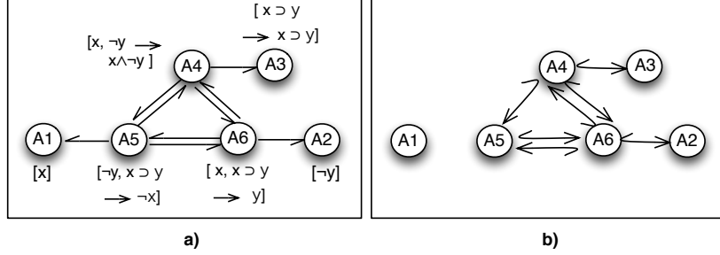
Figure 4: Classical Logic argumentation: attack graph (a) and defeat attack (b)
