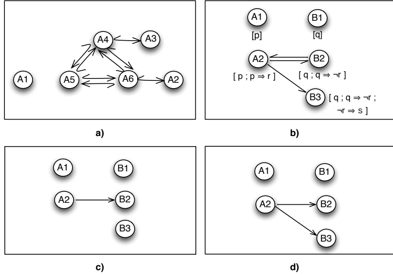
Figure 5: Examples illustrating comparison with critiques of PAFs
