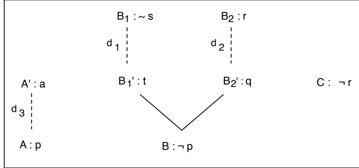
Figure 1: ASPIC^+ arguments and their conclusions, with dashed and solid lines respectively representing application of defeasible and strict inference rules.
