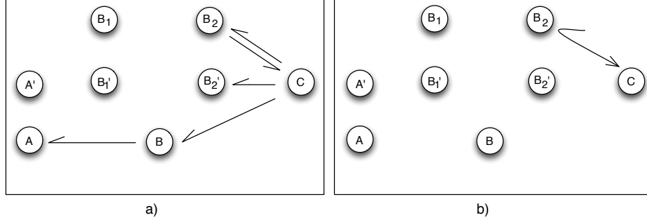
Figure 2: Example 4's ASPIC^+ attack graph shown in a). Note that the dashed and solid lines representing application of defeasible and strict inference rules have been removed. The defeat graph (see Example 6) is shown in b).
