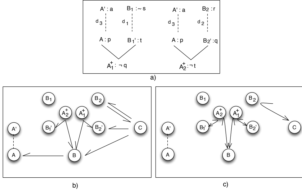
Figure 3: Example 7's arguments A_1^+ and A_2^+ built from transpositions of the strict rule t, q \rightarrow \neg p are shown in a). ASPIC^+ attack graph shown in b). A possible defeat graph is shown in c).
