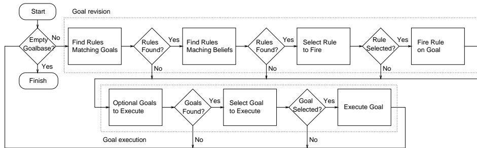
Figure 2: The deliberation cycle of the 3APL interpreter.
